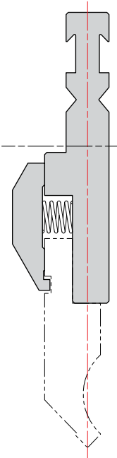
Attache BYSTRONIC type R, RF, RF-A, S
