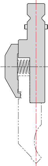
Attache WILA, TRUMPF
